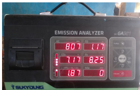
Figure 2. Gas analyzer
