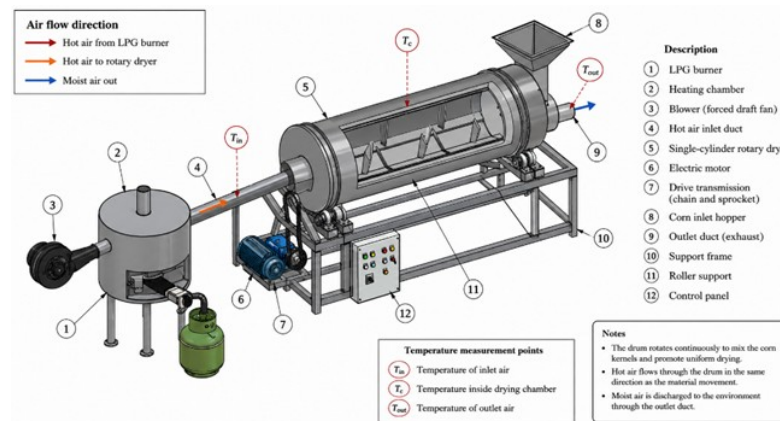
Figure 1. Schematic of the experimental setup for corn drying in an LPG-fired single-cylinder rotary dryer
